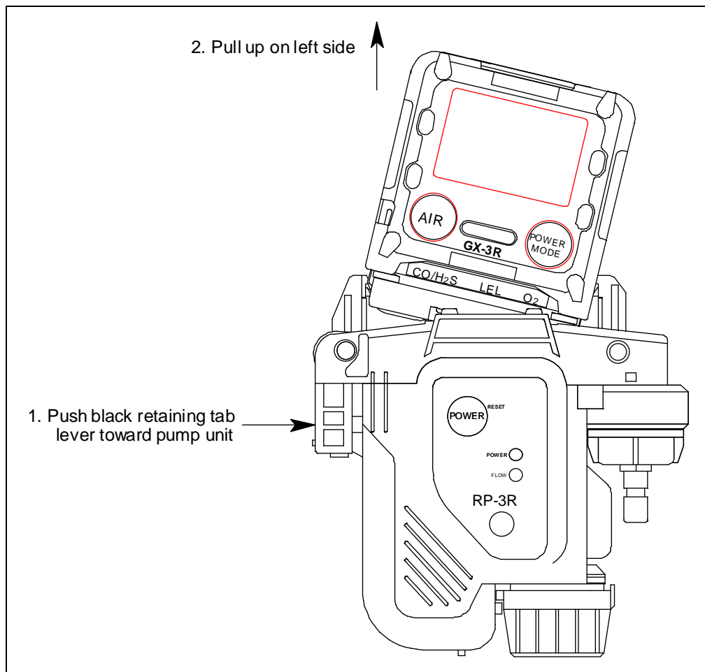
Figure 4: GX-3R Removal
