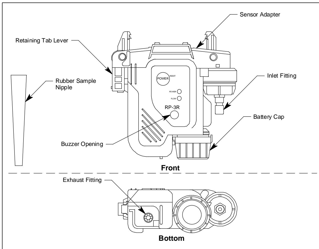
Figure 1: Component Location
